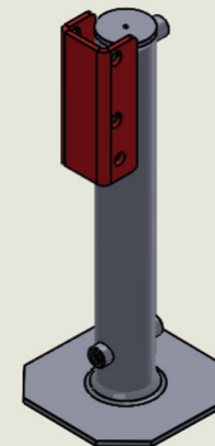
C-Channel Bracket
