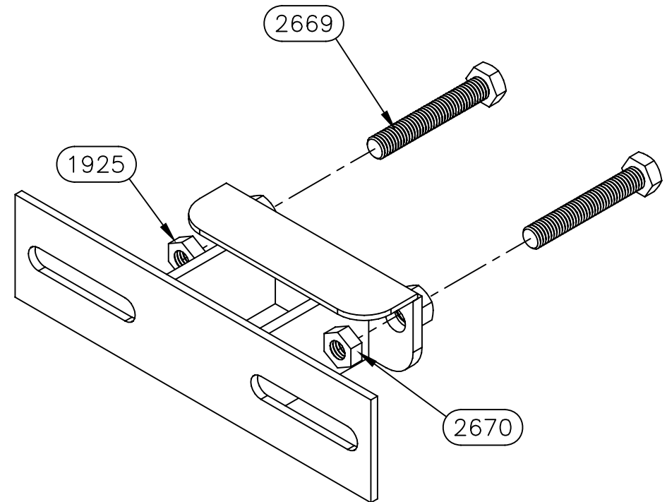
NEW STYLE 1925 BRACKET USED ON ALL CENTER CYLINDER SLIDES (EXCEPT NORCO/EQUALIZER HYBRID) STARTING IN NOVEMBER 2010 THIS REPLACES THE OLD ONE AND REQUIRES (2) 2669 BOLTS, AND (2) 2670 NUTS, THAT ARE USED AS STOPS FOR THE SLIDE
