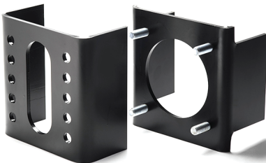
Leg Mount Brackets For E450 & E350 For Chassis
